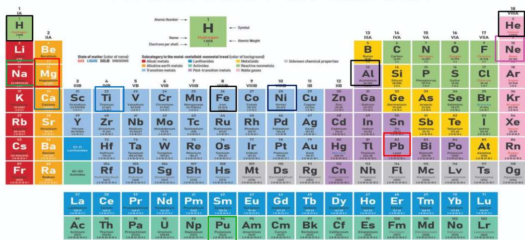
Periodic Table of the Elements
